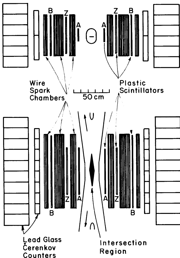
Figure 8. CCR apparatus, CERN ISR.
